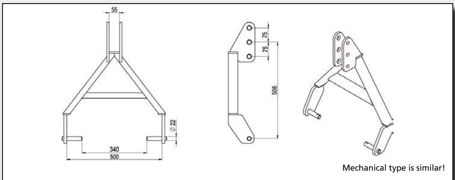
Three-point linkage CAT I N
