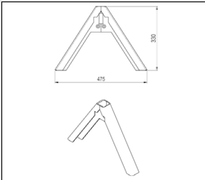
A-frame: CAT Communal
